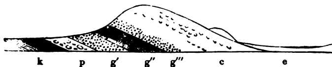
Diagram IX. k. Kimmeridge clay. p. Portland rock. g'. Lower green-sand. g''. Gault. g'''. Upper green-sand. c. Chalk. e. Eocene strata.
