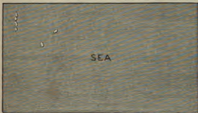
Diagram XIV. Land submerged 1000 feet.
