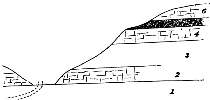
Diagram I. 1. Sandy clay. 2. Rock, 20 feet. 3. Wet clay. (Spring of water here.) 4. Ovenstone or soft sandstone. 5. White sand, 6 feet. 6. White stone. The Road to Hopercroft's Holt is dotted.
