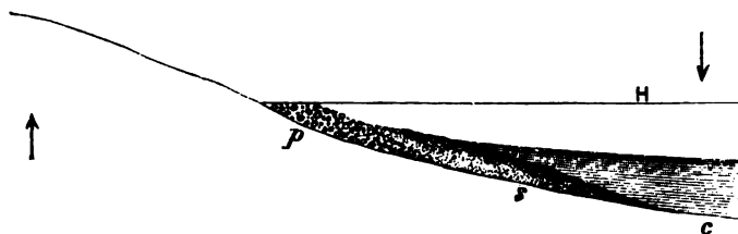
Diagram XXIII. Sedimentary shore deposits.
