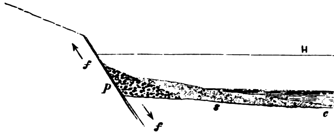
Diagram XXIV. Deposits against a fault.
