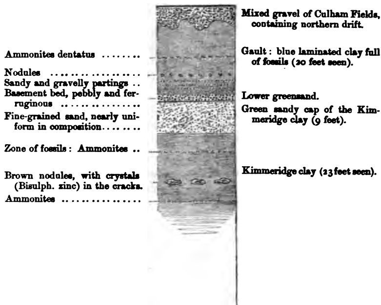
Diagram CXCVI. Section of the Strata at Culham, south of Oxford.
